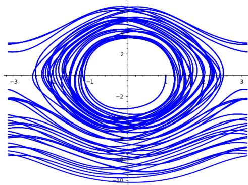
Figure 3.1: The driven pendulum obtained from numerically integrating the Hamilton equations. The graph is not identical to the one in the book, because of the inherent chaotic behavior.
