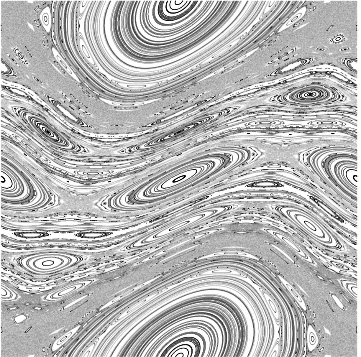
Figure 3.3: The standard map with K = 0.6 .
